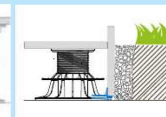
Finishing with a buttress
