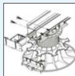
Joist extremity
