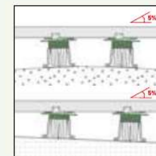
Self-levelling head.
